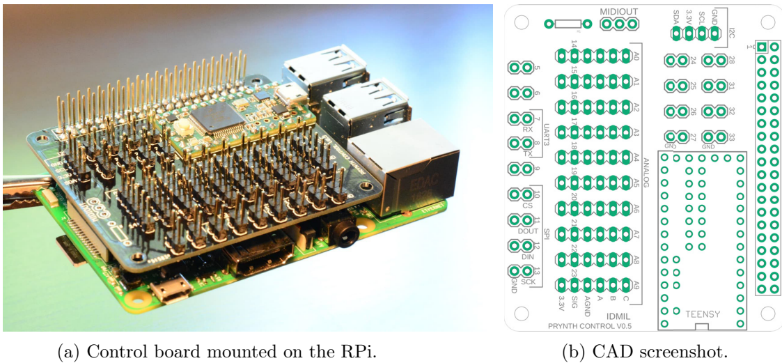
Fig. 5.4 Control board.
