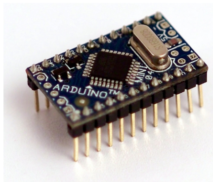
(a) Arduino mini 04 used in the Sopranos and the Tenor T-Sticks.
