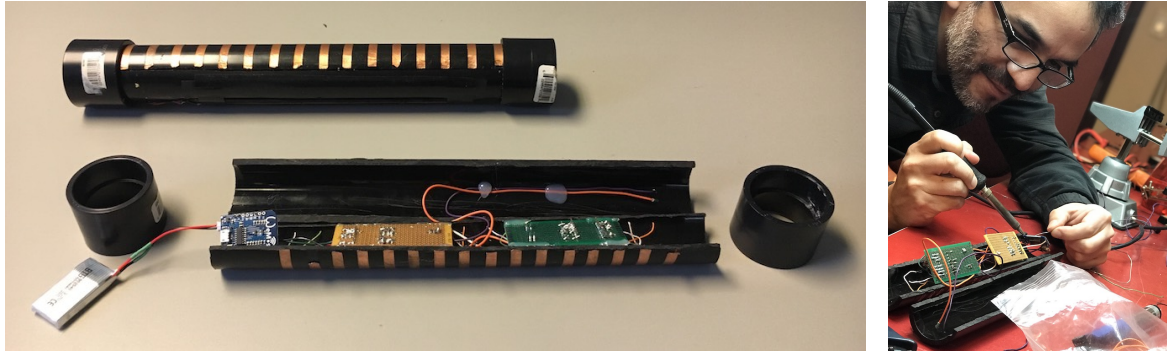
(a) Top: Sopranino 2G-172, Bottom: Sopranino 2GW-181 under construction. Notice the different boards. The brown perfboard holds the original electronics while the green one is the reconstructed one.
