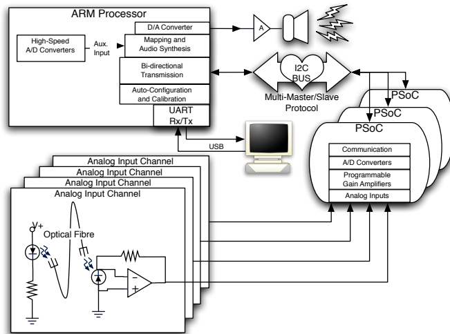
Figure 1. Example system configuration showing fibre optic sensor-based interface.
